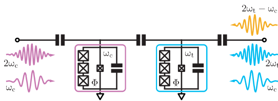
Fig. 5. Schematic for possible realization of the bias-preserving CX gate with superconducting circuits. Here, the Kerr nonlinear oscillators (of frequencies \omega_c and \omega_t ) are implemented with superconducting nonlinear asymmetric inductive elements or SNAILs (38, 39). A SNAIL can be biased with an external magnetic field so that it has both three- and four-wave mixing capabilities. It can therefore be used to implement the two-photon driven Kerr nonlinear oscillator and realize a cat qubit with biased-noise channel (19). The Hamiltonian in Eq. 26 can be simplified as \hat{H} = -K\hat{a}_c^{\dagger 2}\hat{a}_c^2 - K\hat{a}_t^{\dagger 2}\hat{a}_t^2 + K\beta^2(\hat{a}_c^{\dagger 2} + \text{h.c.}) + K\alpha^2 \cos(\phi(t)) (e^{i\phi(t)}\hat{a}_t^{\dagger 2} + \text{h.c.}) - (K\alpha^2 \sin(\phi(t))/\beta) (ie^{i\phi(t)}\hat{a}_t^{\dagger 2}\hat{a}_c + \text{h.c.}) + (K\alpha^4/2\beta) \sin(2\phi(t)) (i\hat{a}_c^{\dagger} + \text{h.c.}) - (K\alpha^4 \sin^2(\phi(t))/\beta^2)\hat{a}_c^{\dagger}\hat{a}_c^{\dagger} - \phi(t)\hat{a}_t^{\dagger}\hat{a}_t^{\dagger}/2 + (\phi(t)/4\beta)\hat{a}_t^{\dagger}\hat{a}_t^{\dagger}(\hat{a}_c^{\dagger} + \text{h.c.}) . By expressing the Hamiltonian in this form, the drives required to realize the Hamiltonian become immediately clear. First, a drive to the control cavity (fixed amplitude and phase) centered at 2\omega_c is required for the two-photon term driving the control cavity via three-wave mixing. Next, a drive to the target cavity with time-dependent amplitude at 2\omega_t results in the two-photon term driving the target cavity via three-wave mixing. An additional drive 2\omega_t - \omega_c (time-dependent amplitude and phase) is applied to the target cavity to realize the coupling terms \propto \hat{a}_t^{\dagger}\hat{a}_c in Eq. 26. A drive applied directly to the control cavity centered at \omega_c with time-dependent phase and amplitude realizes the single-photon drive to the control cavity. A final drive to the target cavity at \omega_c with time-dependent amplitude and phase realizes the last term in the Hamiltonian (40).
