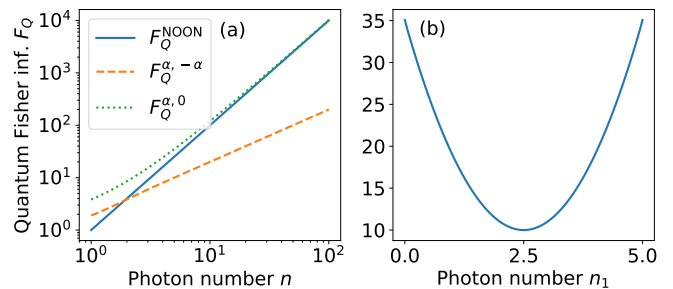
Figure 3. Quantum Fisher information in swap-test interferometry. (a) Scaling of the quantum Fisher information with the total photon number at the input for NOON states ( F_Q^{\text{NOON}} , solid blue line), entangled coherent states with \alpha_1 = -\alpha_2 ( F_Q^{\alpha, -\alpha} , dashed orange line), and entangled coherent states with \alpha_2 = 0 ( F_Q^{\alpha, 0} , dotted green line). The total photon number for entangled coherent states is \alpha_1^2 + \alpha_2^2 . (b) Quantum Fisher information for entangled coherent states with the total photon number n = 5 for different partitions of the total energy between the two modes. We assume two real coherent-state amplitudes \alpha_1 = \sqrt{n_1} , \alpha_2 = -\sqrt{n - n_1} .
