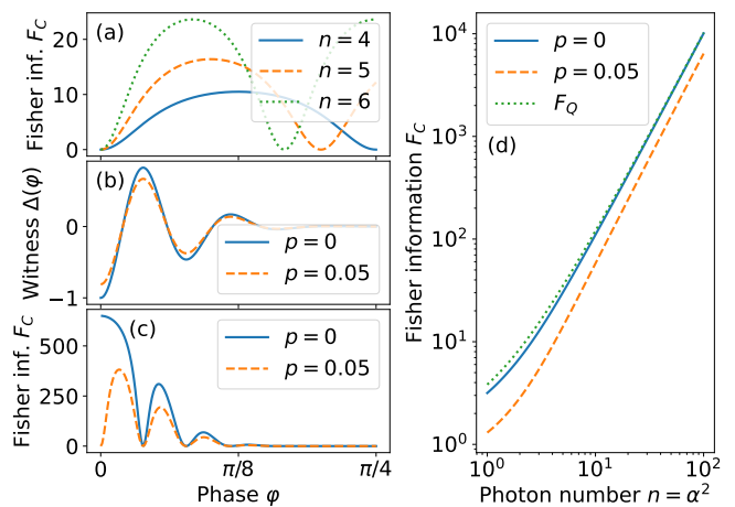
Figure 5. Fisher information with ancilla phase-flip errors. (a) Classical Fisher information for NOON states with n = 4 (solid blue line), n = 5 (dashed orange line), and n = 6 (dotted green line) with phase-flip probability of 5 %. (b) Overlap witness for coherent states with \alpha_1 = \alpha, \alpha_2 = 0 with \alpha = 5 in the ideal case ( p = 0 , solid blue line) and with phase flips (probability p = 0.05 , dashed orange line). (c) Classical Fisher information for the overlap witness shown in (b). (d) The maximum classical Fisher information (for coherent states with \alpha_2 = 0 , optimized over the phase \varphi ) as a function of the photon number n = \alpha^2 ; the quantum Fisher information is plotted as well (dotted green line).
